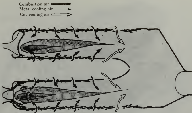
FIGURE 1-49. Airflow through a can-annular chamber.
